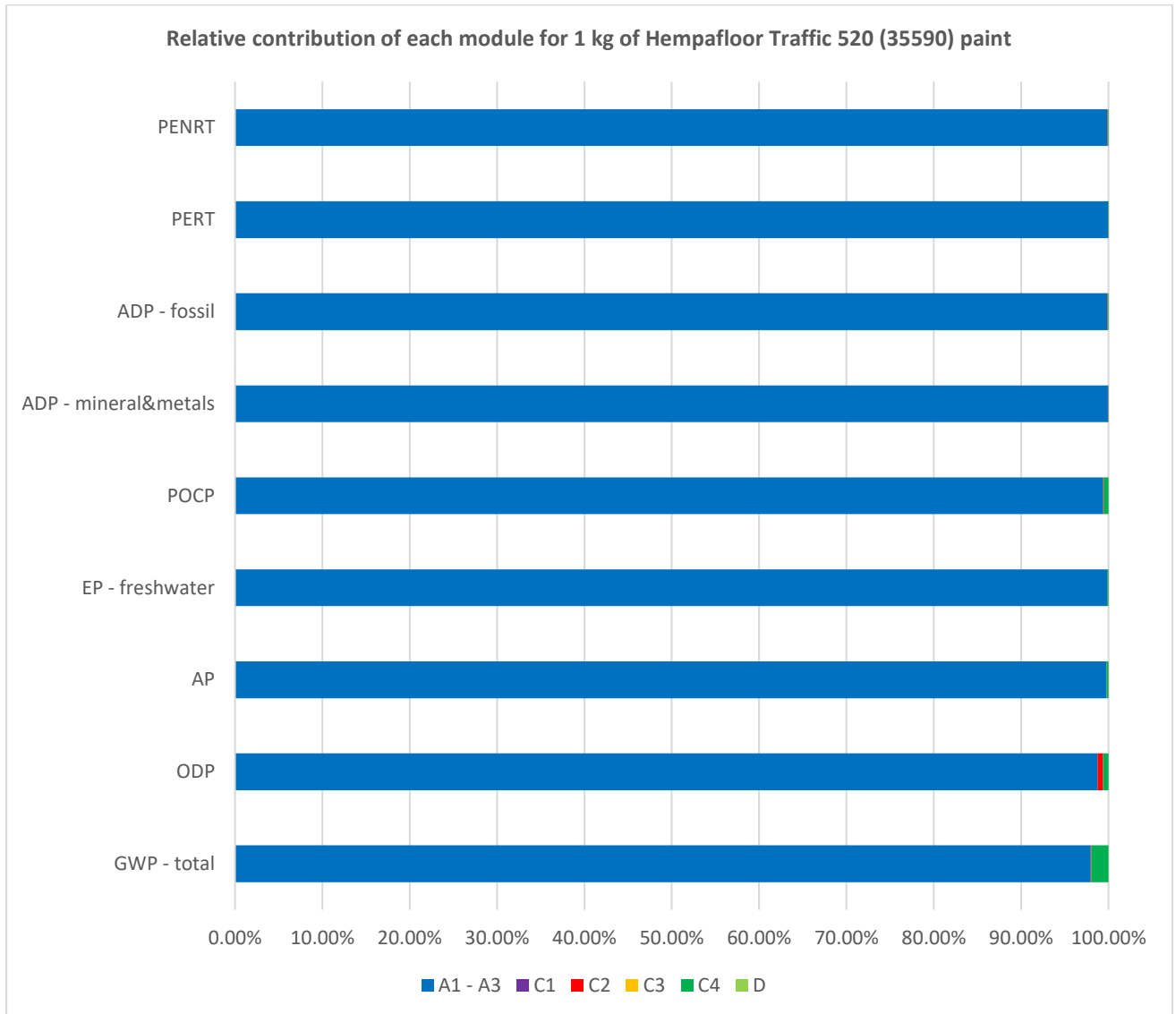
Figure 1: Relative contribution of each module for 1 kilogram of Hempafloor Traffic 520 (35590) paint.
