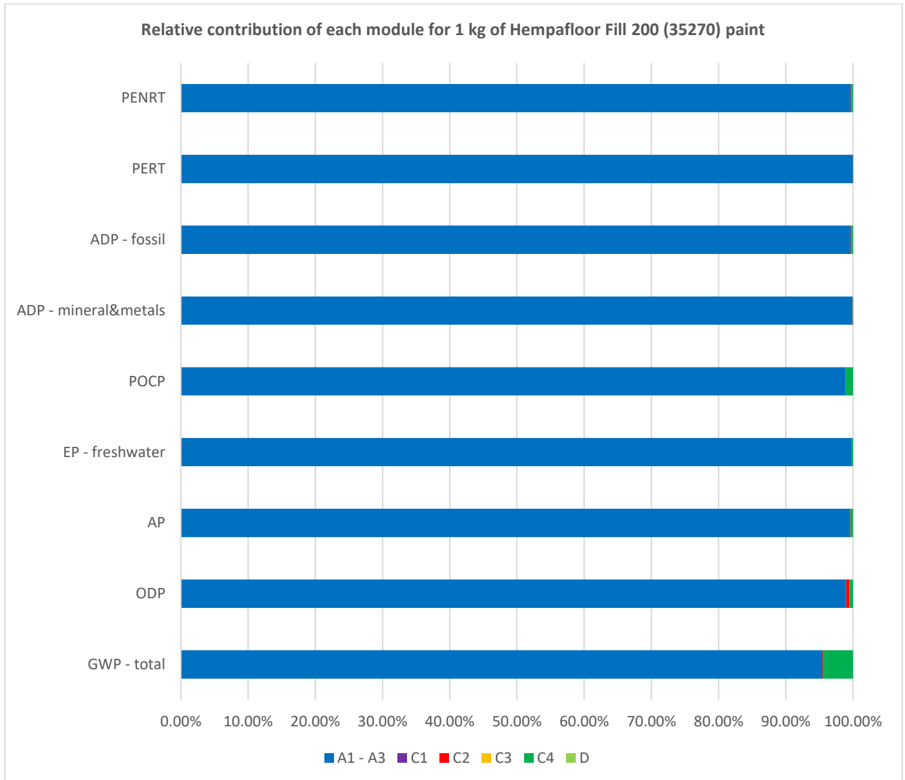
Figure 1: Relative contribution of each module for 1 kilogram of Hempafloor Fill 200 (35270) paint.
