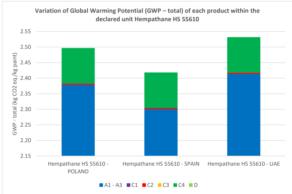
Figure 2: Variation of Global Warming Potential (GWP – total) of each product within the declared unit, 1 kilogram of Hempathane HS 55610 paint.
