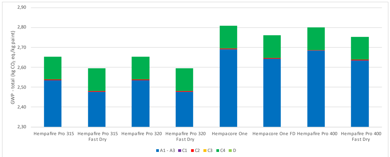
Figure 2: Variation of Global Warming Potential (GWP – total) of each product within the declared unit, 1 kilogram of solvent-borne PFP (Passive Fire Protection) paint.
