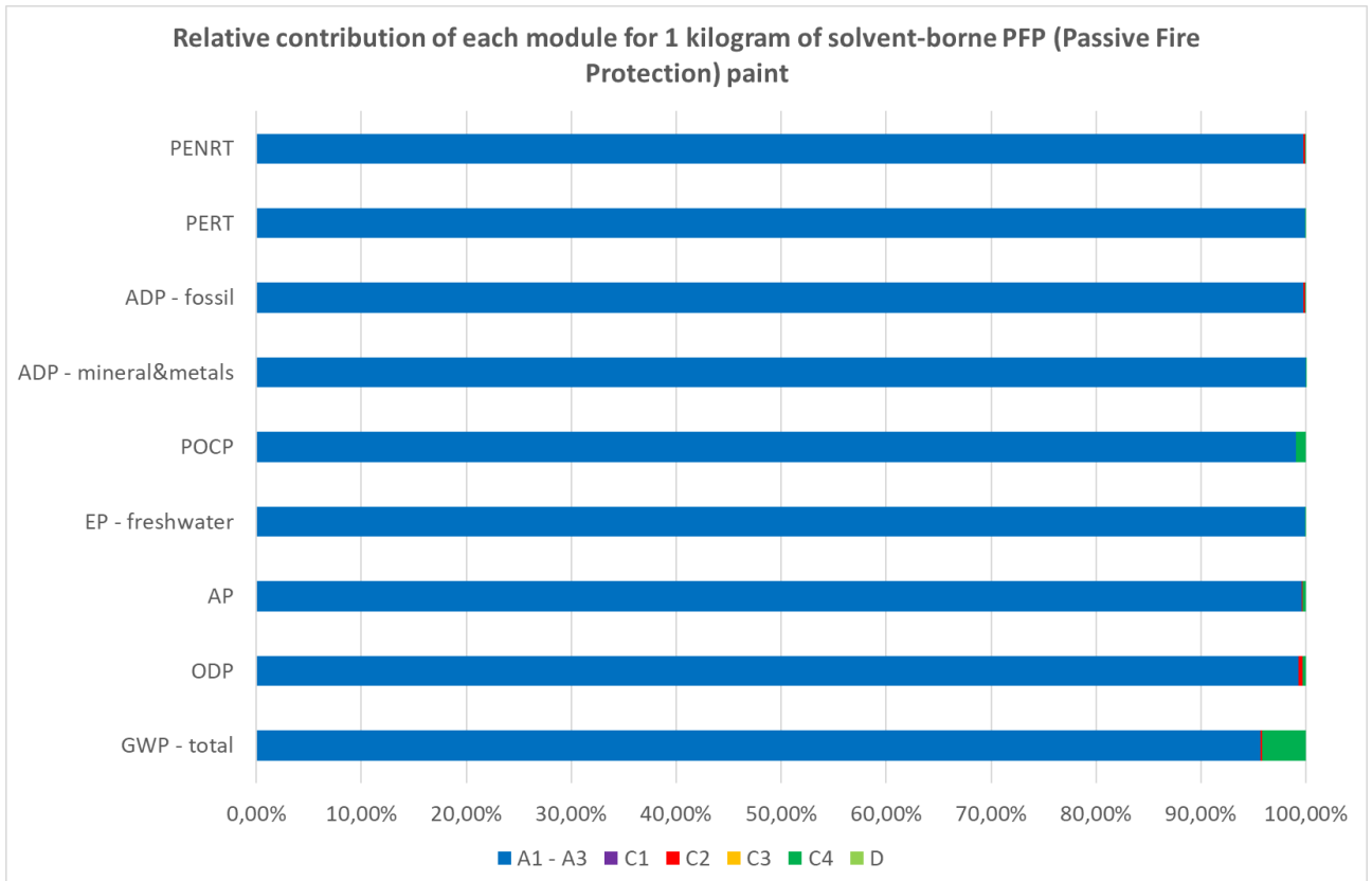
Figure 1: Relative contribution of each module for 1 kilogram of solvent-borne PFP (Passive Fire Protection) paint.
