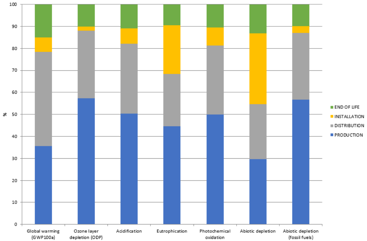
Figure 4. CUPACLAD® 101 System Life Cycle Assessment Results.
