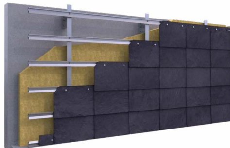
Figure 2. CUPACLAD® 101 Logic system.
