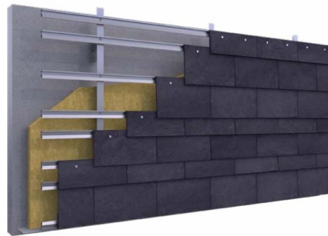
Figure 3. CUPACLAD® 101 Random system.
