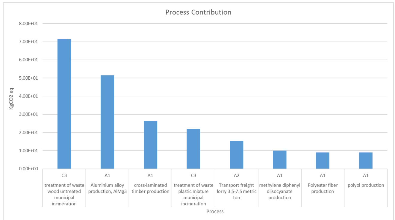
Chart 1: Process contribution chart for Banqs Sofa
