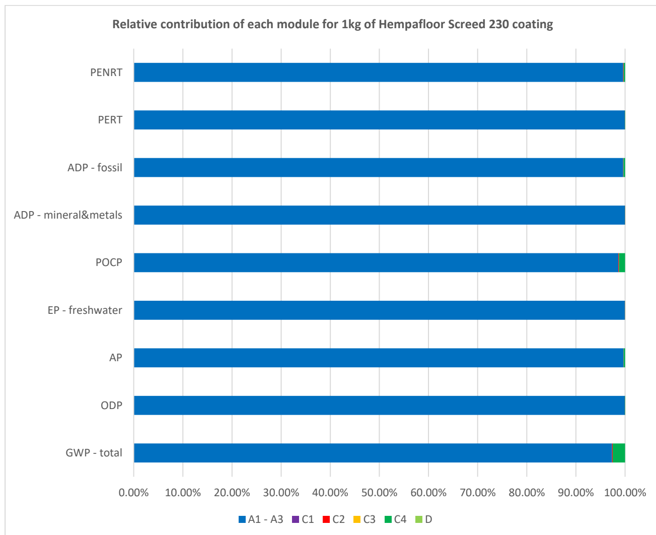
Figure 1: Relative contribution of each module for 1 kilogram of Hempafloor Screed 230 coating.
