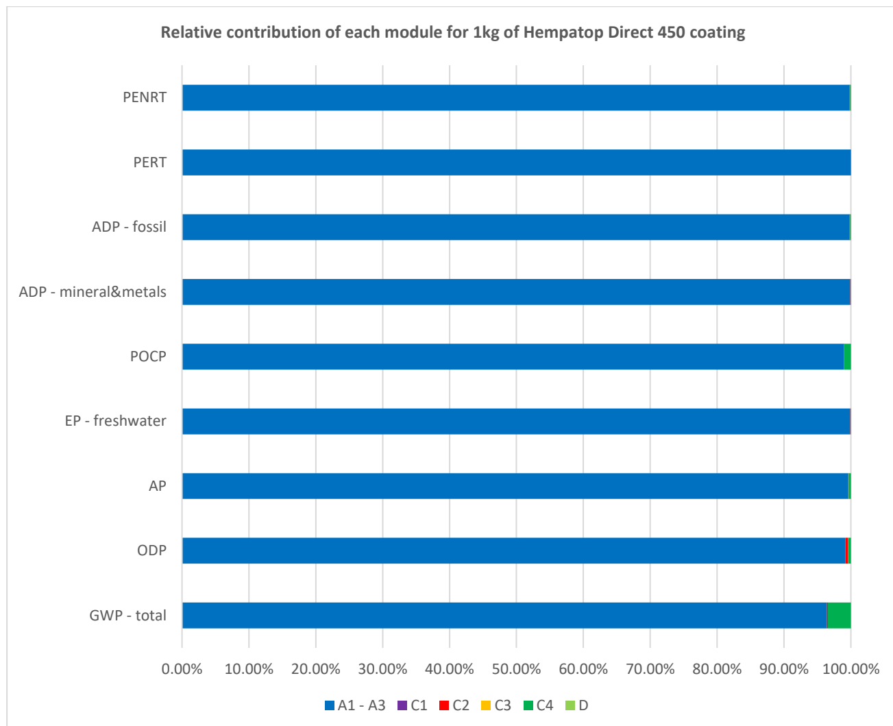
Figure 1: Relative contribution of each module for 1 kilogram of Hempatop Direct 450 coating.
