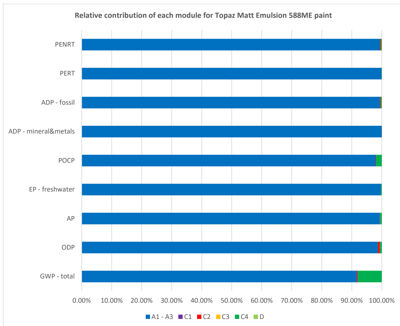
Figure 1: Relative contribution of each module for 1 kilogram of Topaz Matt Emulsion 588ME paint.
