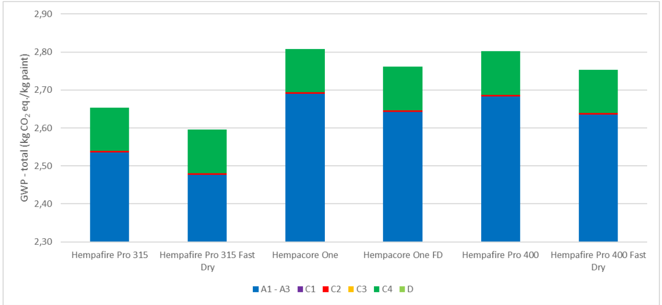
Figure 2: Variation of Global Warming Potential (GWP – total) of each product within the declared unit, 1 kilogram of solvent-borne PFP (Passive Fire Protection) paint.
