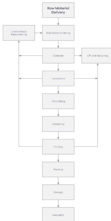
Amtico Production Process
